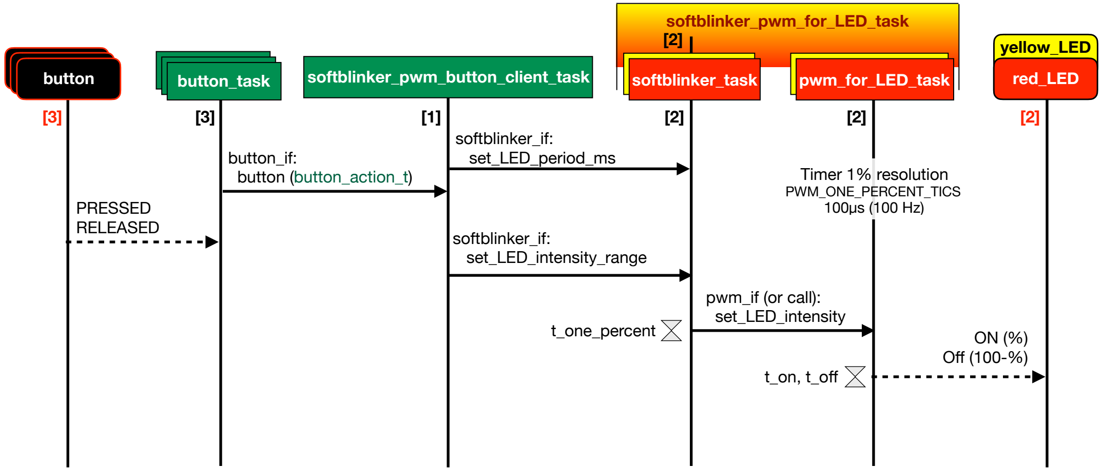
_Softblinker_PWM: Message Sequence Chart (MSC) Øyvind Teig (Trondheim, 7.2020)
