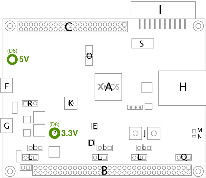
Figure 1: xCORE-200 explorerKIT block diagram
