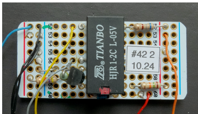
R4 R5 T1 RELAY R2
