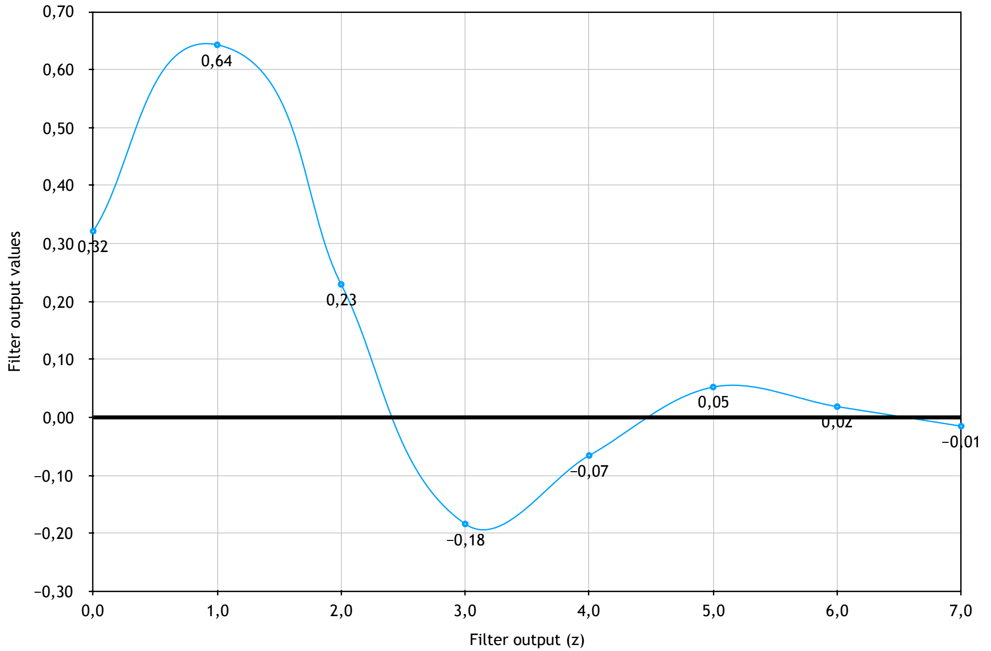
XMOS AN00209_app_design. Impulse response
