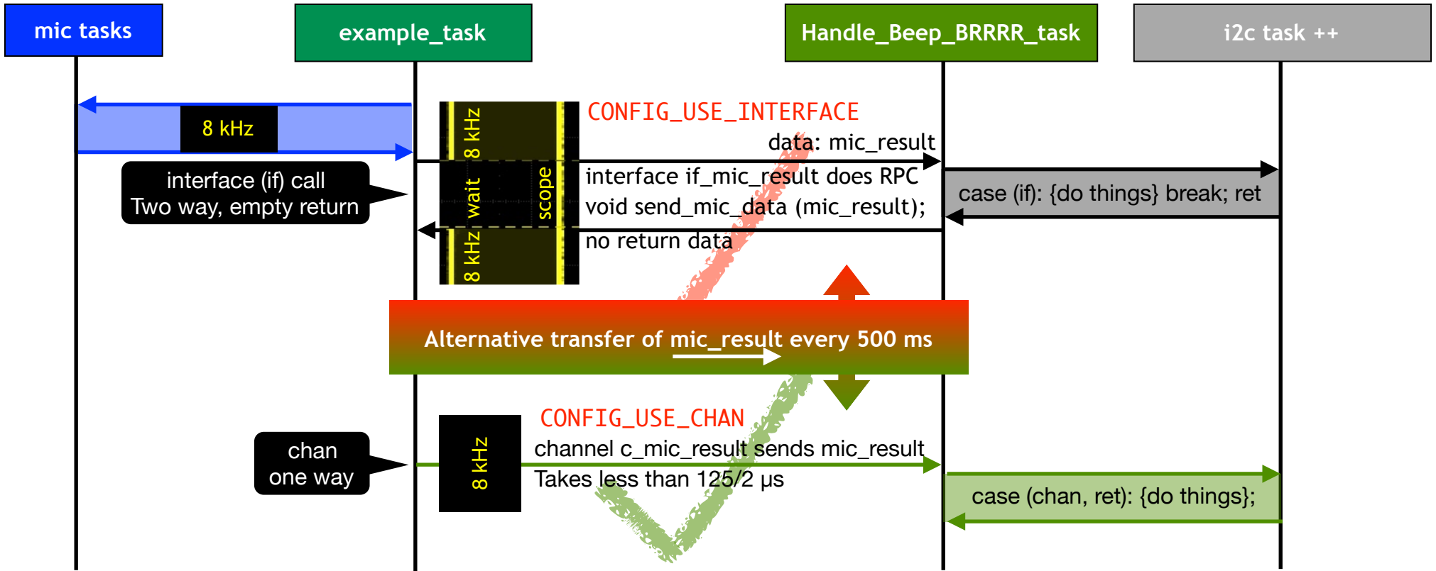
interface vs. channel during critical timing: Message Sequence Chart (MSC) Øyvind Teig (Trondheim, 9.2021)
