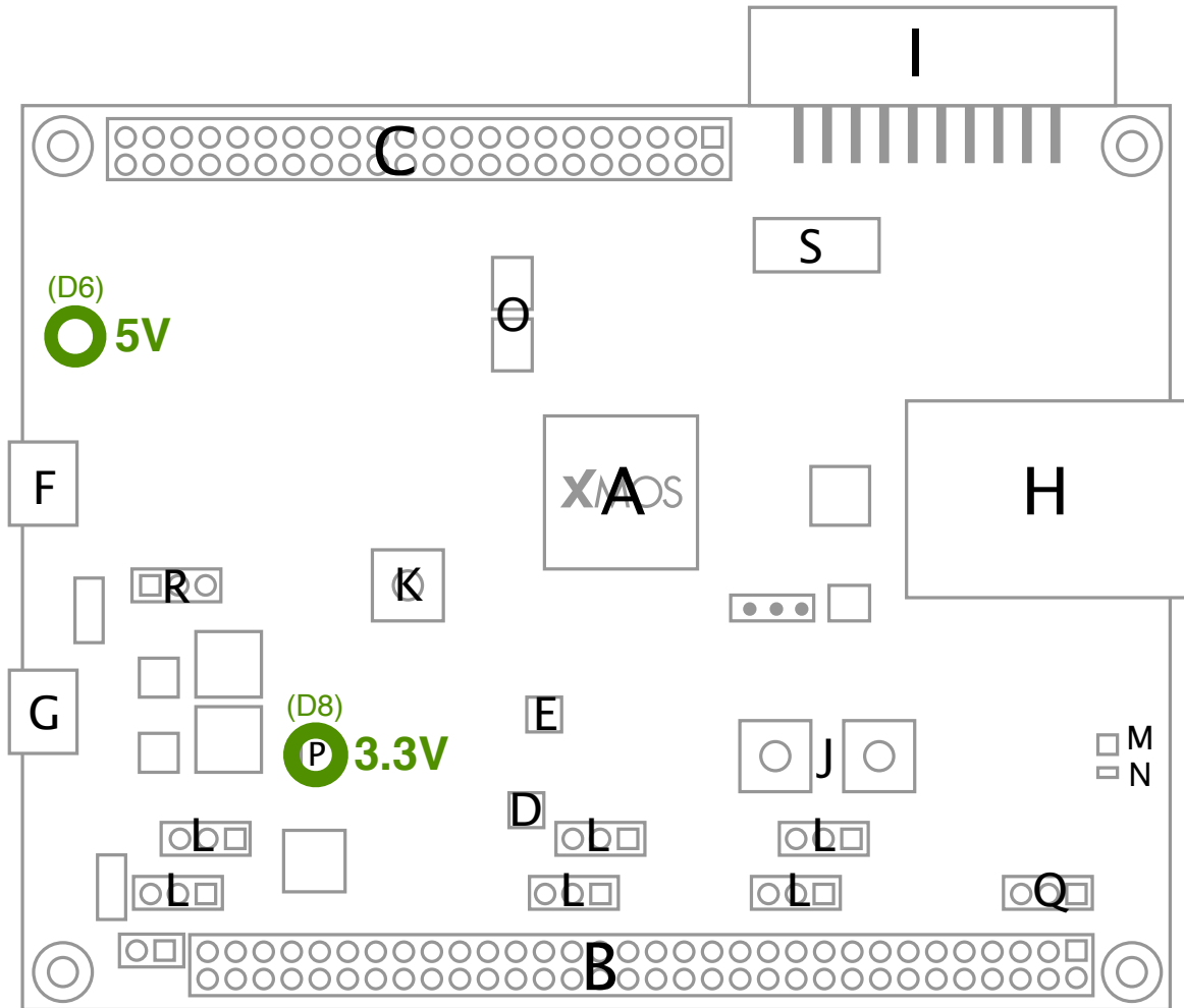
Figure 1: xCORE-200 explorerKIT block diagram
